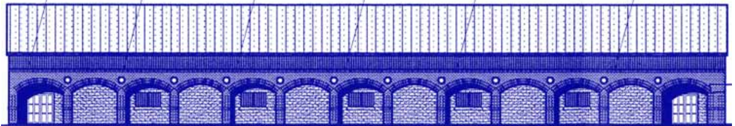
East elevation with doors at the two ends. Arch design is used to keep the Indian style.
